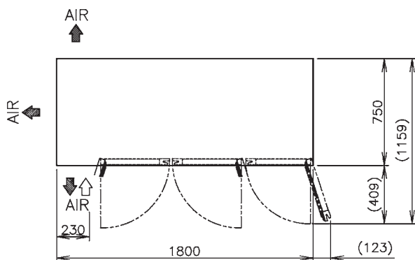
VIEW A(1/10)
