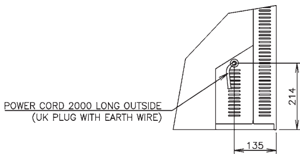
VIEW A(1/10)
