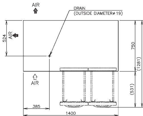
VIEW A (1/10)
