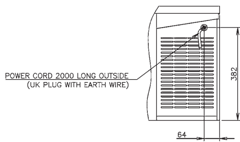
VIEW A (1/10)
