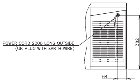
VIEW A (1/10)
