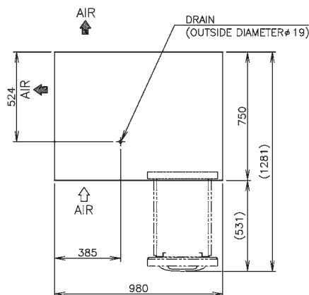
VIEW A (1/10)
