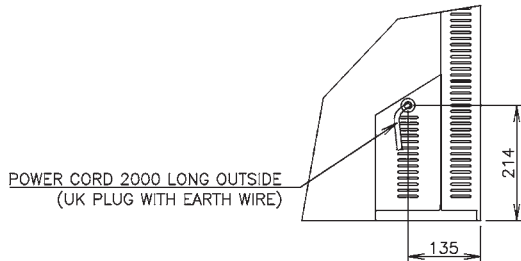
VIEW A(1/10)
