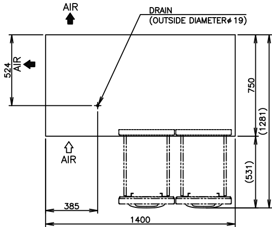
VIEW A (1/10)
