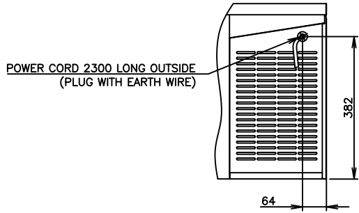
VIEW A (1/10)
