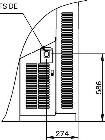
VIEW A (1/10)
