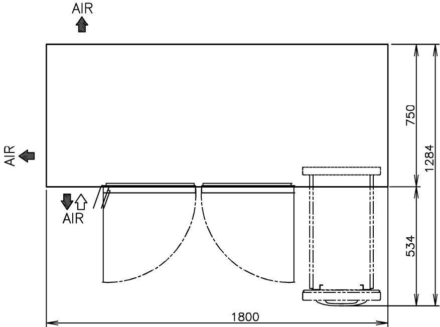
VIEW A (1/10)
