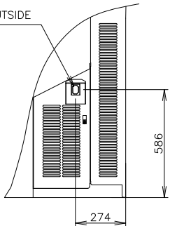
VIEW A (1/10)
