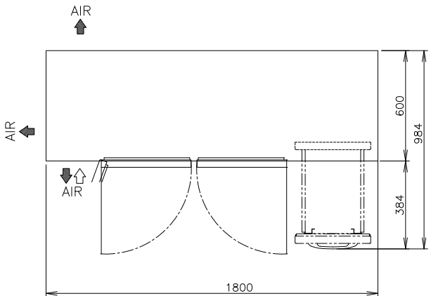
VIEW A (1/10)
