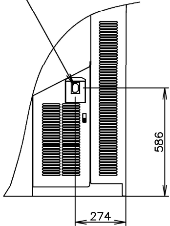
VIEW A (1/10)
