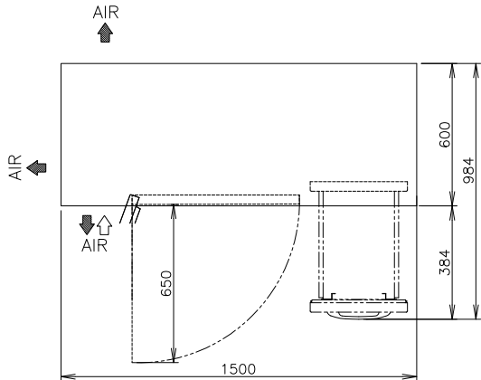
VIEW A (1/10)
