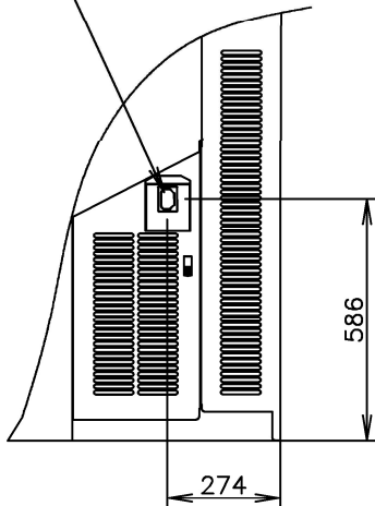
VIEW A (1/10)
