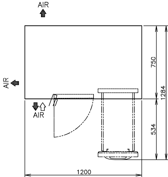
VIEW A (1/10)
